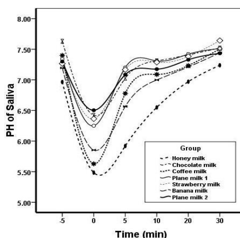
Figure 2. Course of changes in salivary pH at different time intervals
