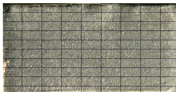
Figure 4. Broken specimen without soldering at \times 10.5 magnification
