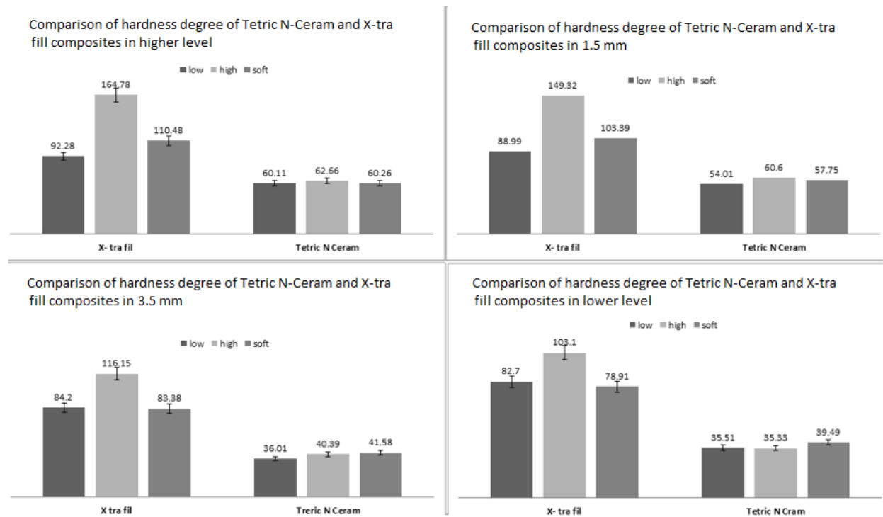
Figure 3. Comparison of the Vickers hardness number(kg/m 2 ) of X-tra fil and Tetric N-Ceram in higher and lower levels and in 3.5mm and 1.5mm in depth
