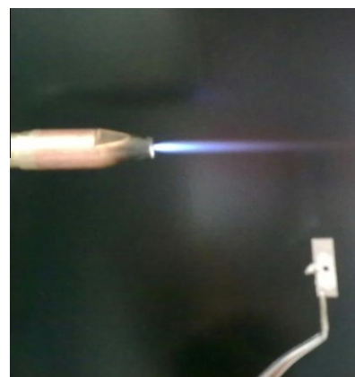
Figure 1. Soldering phase
